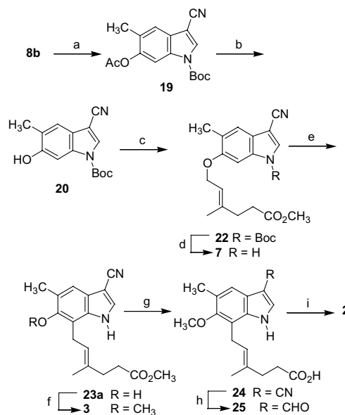
Scheme 4. Reagents and conditions: (a) (Boc) 2 O, 2% DIEA in MeCN; (b) Na 2 CO 3 , NaHCO 3 , aq. Dioxane; (c) 21b , K 2 CO 3 , acetone, 25 °C; (d) NaOMe, MeOH; (e) Montmorillonite KSF, toluene, reflux, 20 min; (f) diazomethane, MeOH, ether, 25 °C; (g) LiOH, MeOH, H 2 O; (h) i. Dibal-H, CH 2 Cl 2 , –78 °C; ii. Tartaric acid, H 2 O; (i) NH 3 , NaCN, MnO 2 , 2-propanol, 0–5 °C.
