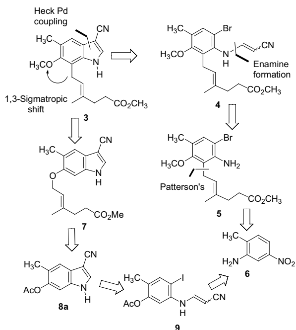
Scheme 1. Retrosynthetic strategies for 3 .
