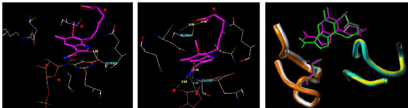
Figure 6. Docking of 2 into Chinese Hamster IMPDH. (A) The indole 2 (magenta) built via modification of MPA inside Chinese hamster IMPDH active site. Note the steric interaction between the C2 on indole and the side chain of the Thr-333. The IMP is highlighted in orange. (B) The model illustrated in A after energy minimization. Water molecules are shown as red spheres. The distances shown are attributed to the H bonding of the 3-carboxamide and the side chain carboxylic acid group with the active site. (C) Active site loop (orange tube) and flap (cyan tube) in A (before minimization) compared with B. The loop in B is shown in white and the flap is shown in yellow. The indole 2 and Thr-333 are colored magenta (before minimization) and green (after minimization). Note the slight movement of the loop toward the modeled ligand 2 to establish new H-bonds with the amide group.
