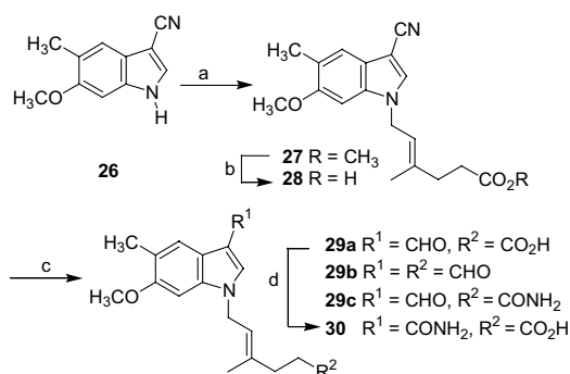
Scheme 5. Reagents and conditions: (a) 21c , \text{K}_2\text{CO}_3 , acetone, reflux; (b) KOH, MeOH, \text{H}_2\text{O} ; (c) i. Dibal-H, \text{CH}_2\text{Cl}_2 , 0^\circ\text{C} ; (ii) Rochelle salt; (d) \text{NH}_3 , NaCN, \text{MnO}_2 , 2-propanol, 0 – 5^\circ\text{C} .
