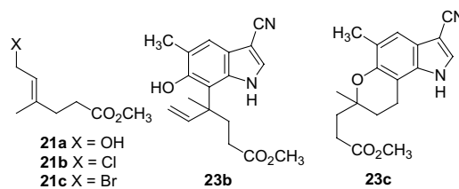
Figure 2. Structure of side chain intermediates ( 21a–21c ) and products from attempts of 1,3-sigmatropic rearrangement under different conditions ( 23b and 23c ).
