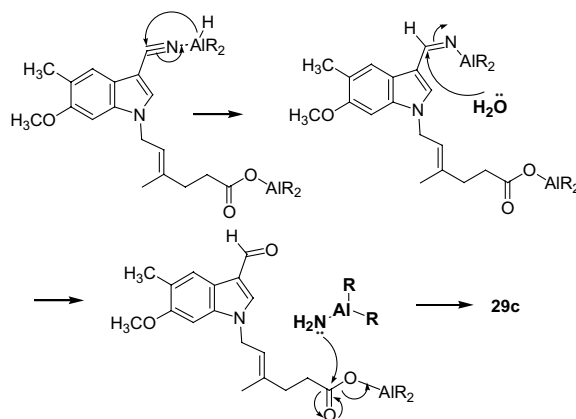
Figure 3. Proposed mechanism for formation of 29c .
