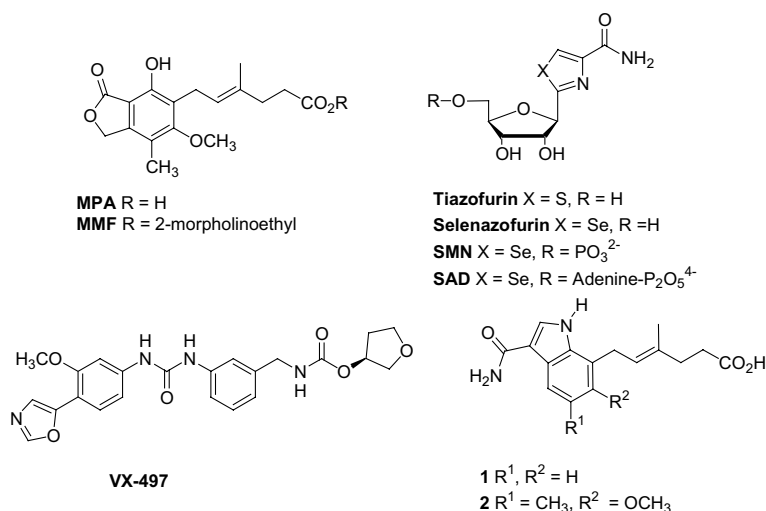
Figure 1. Inhibitors of human IMPDH and indole analogs of MPA.
