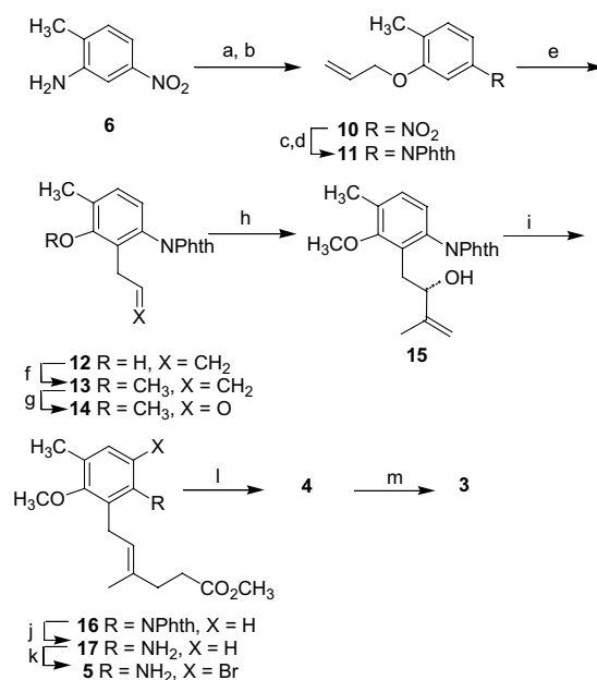
Scheme 2. Reagents and conditions: (a) i. NaNO 2 , H 2 SO 4 , 0–5 °C; ii. H 2 SO 4 , 120 °C, 20 min; (b) allyl Br; K 2 CO 3 , acetone, reflux; (c) SnCl 2 ·2H 2 O, EtOAc, 65–70 °C; (d) phthalic anhydride, DMF, reflux; (e) N,N -diethylaniline, 200 °C; (f) (CH 3 ) 2 SO 4 , K 2 CO 3 , acetone, reflux; (g) i. O 3 , CH 2 Cl 2 , MeOH, Pyridine, –78 °C; (ii) DMS; (h) isopropenyl MgBr, THF, –70 °C; (i) CH 3 C(OCH 3 ) 3 , C 2 H 5 CO 2 H, 100 °C; (j) hydrazine hydrate, MeOH, 25 °C; (k) NBS, DMF; (l) acrylonitrile, 1,4-benzoquinone, Pd(CH 3 CN) 2 Cl 2 , LiCl, THF, 50 °C; (m) Pd(OAc) 2 , P( o -tolyl) 3 , Et 3 N, DMF, 120 °C.
