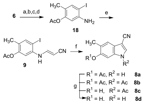
Scheme 3. Reagents and conditions: (a) i. NaNO 2 , H 2 SO 4 , 0–5 °C; (ii) H 2 SO 4 , heat; (b) Ac 2 O, pyridine; (c) SnCl 2 ·2H 2 O, EtOAc, 70 °C; (d) NIS, DMF; (e) cyanoacetaldehyde, TFA, EtOAc; (f) Pd(OAc) 2 , Et 3 N, DMF, heat; (g) K 2 CO 3 , H 2 O, MeOH.
