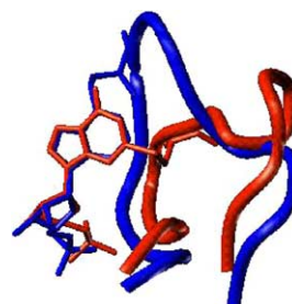
Figure 5. Comparison of the active site loops covalently attached to a substrate site ligand. The Chinese Hamster IMPDH is shown in red and the Human II IMPDH is shown in blue. The IMP C2-Cys-331 adduct seen in the Hamster complex is replaced by a C6-Cys-331 adduct in Human II enzyme. This displaces the loop to the opposite site of purine.
