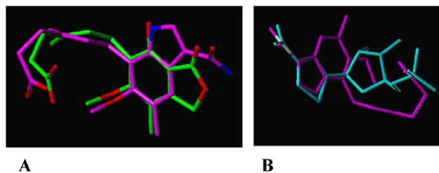
Figure 4. Overlay of 2 with MPA and SAD. The indole 2 is shown in magenta, MPA is green (A), and SMN is shown in cyan (B).
